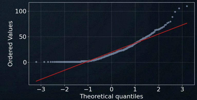
Q-Q Plot (Normality Test)\nNon-Normal Distribution Confirmed
