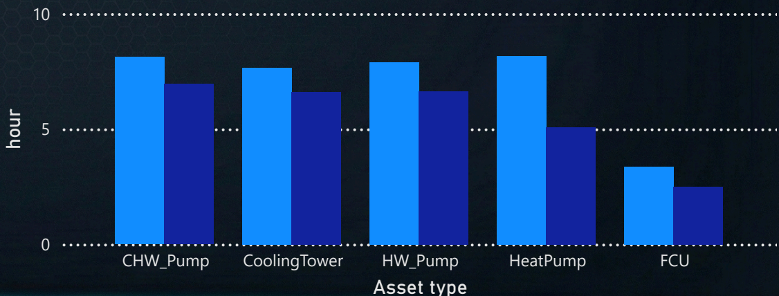
Mean time to repair by asset type and stock status
