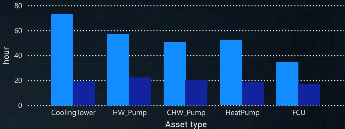
Mean time to repair by asset type and stock status
