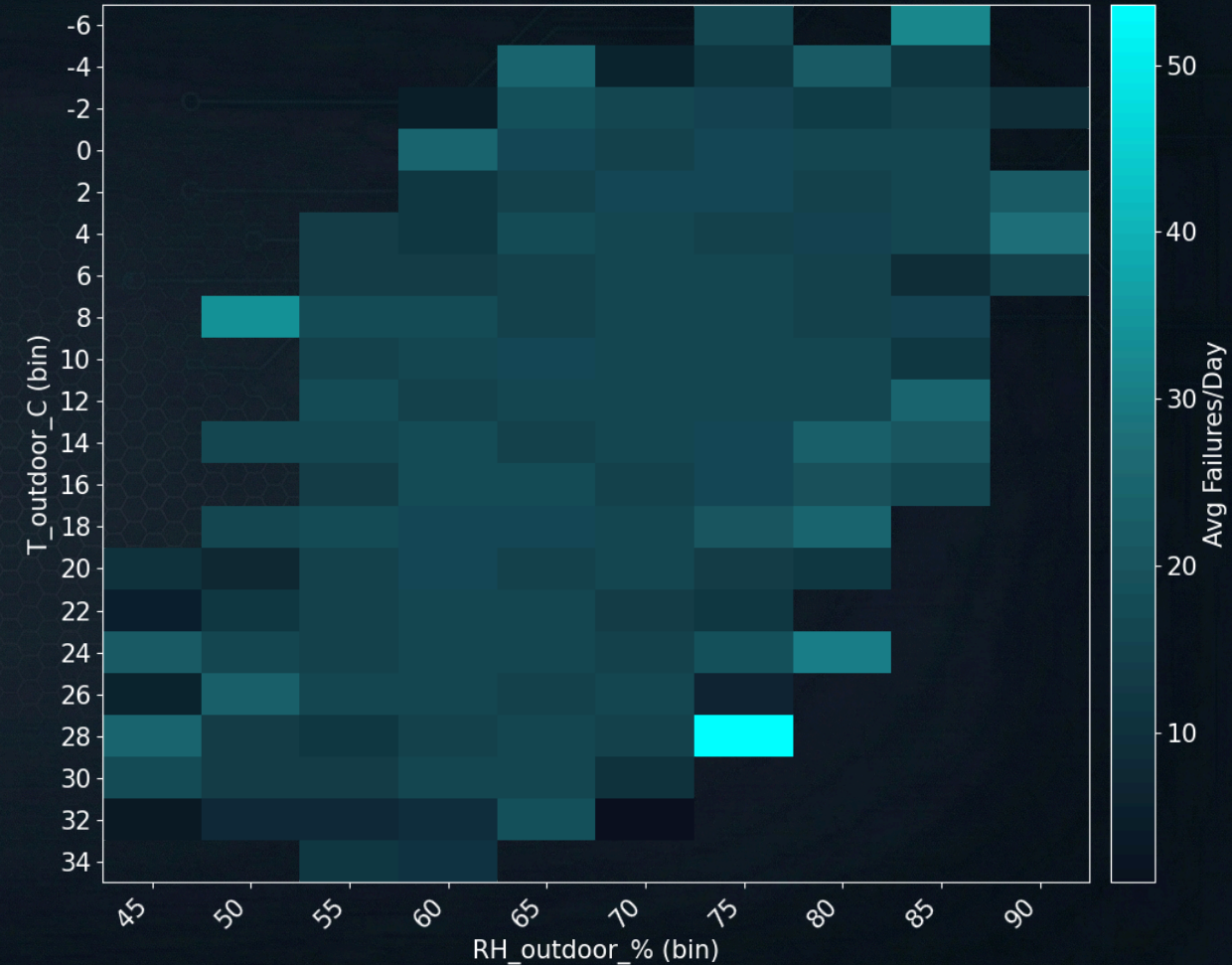
Avg Failures/Day Heatmap — Temperature * Humidity Interaction
