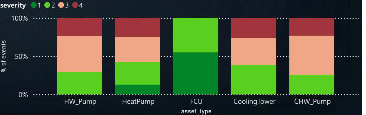
Maintenance Events distribution by asset type and severity
